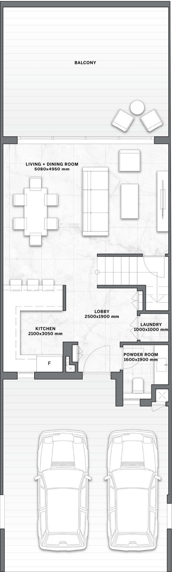
GROUND FLOOR
