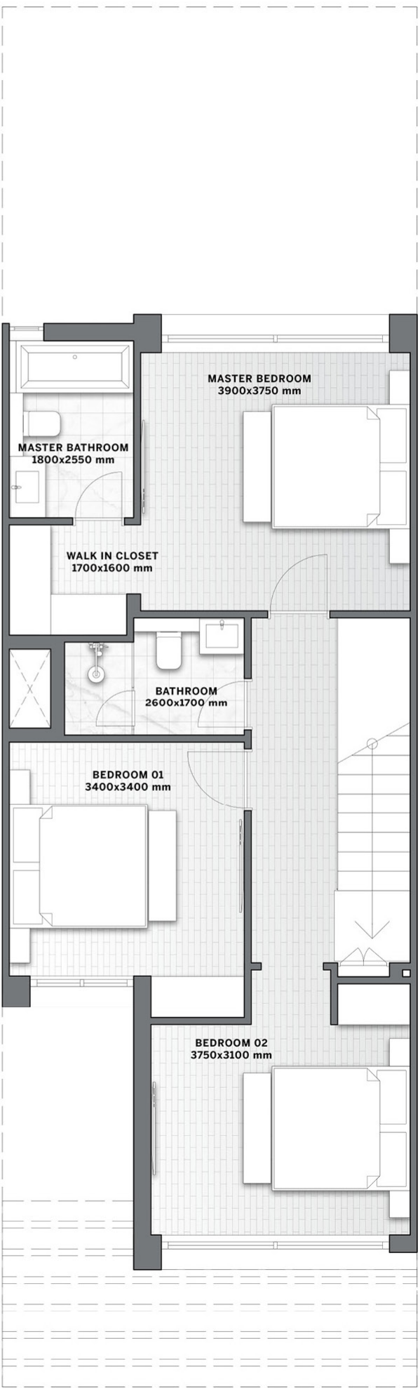
FIRST FLOOR
