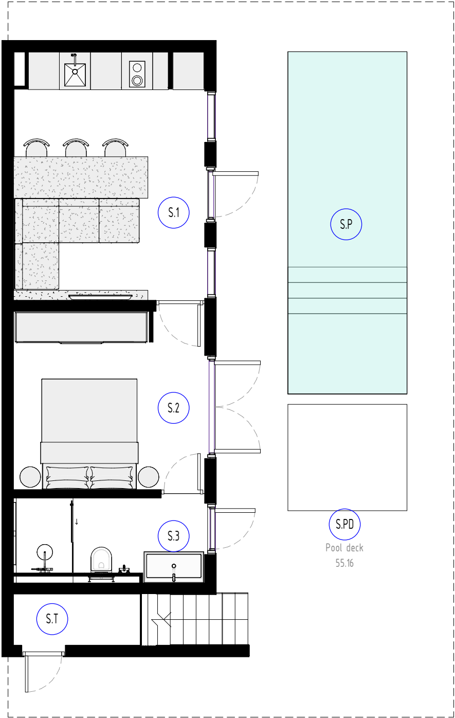
Villa Sc1 1 floor
